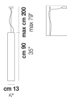
TUBES SP 90
