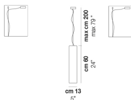
TUBES SP 60
