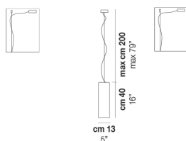
TUBES SP 40
