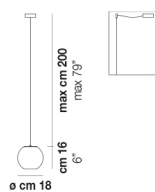
OTO SP 18
