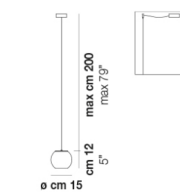
OTO SP 15
